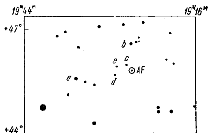
AF Лебеда a = 6,34; b = 6,70; c = 6,87; d = 7,40; e = 7,79.
