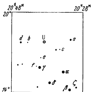
U Дельфина a = 6,27; b = 6,49; c = 6,61; d = 6,76; e = 7,17; f = 7,47.
