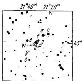
W Лебеда a = 5,34; b = 5,35; c = 5,54; d = 6,11; e = 6,47; f = 6,56; g = 6,70.
